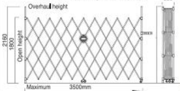
3m x 1,8m Xpanding Barrier system
