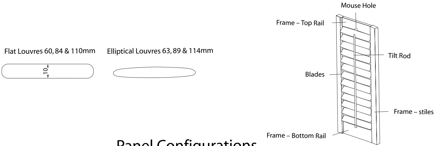
Hinged Panel
